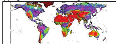
(b) Aridity distribution using SbAI
