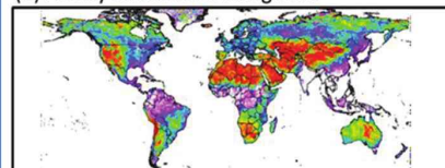
(c) Degraded land (red part)
